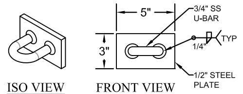
WELDABLE WALL ANCHOR WWA.0503
